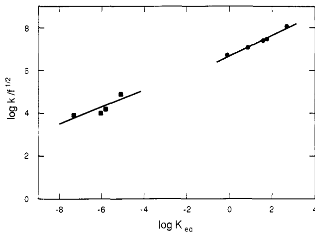
Figure 6. Marcus free energy correlation for the oxidation of singly protonated (■) and fully ionized (●) hydroquinones by 1^{\bullet} and 2^{\bullet} .
